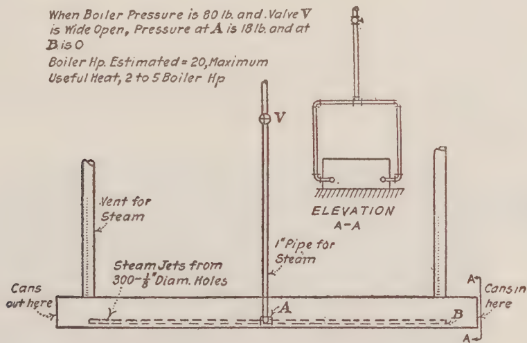
FIG. 2 EXHAUST BOX
